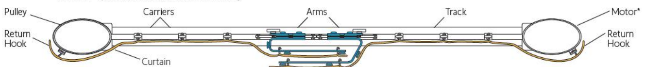
Bottom-up view of track and curtain assembly
