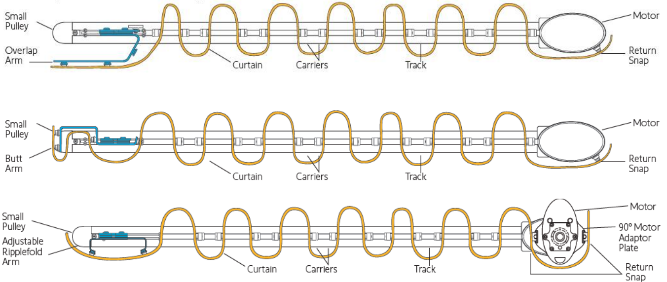
Bottom-up view of track and curtain assembly
