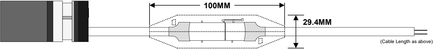
In-Line Connector and Housing Fitted
