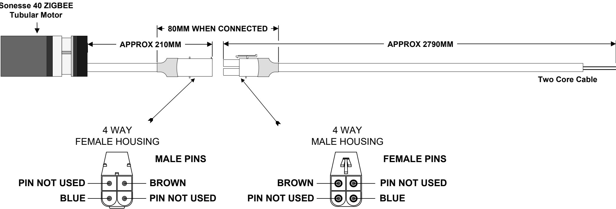
In-Line Connector and Housing Fitted
