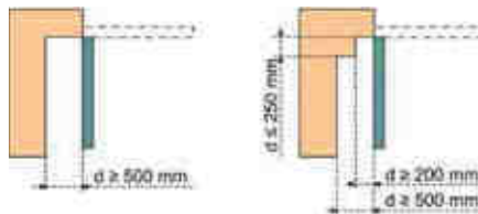
Figure 2 - Mechanical protection
